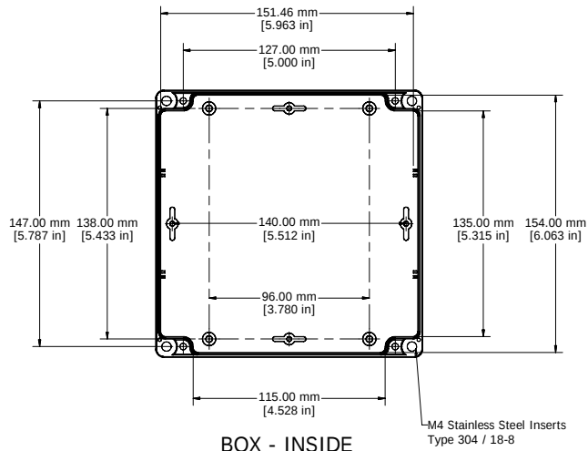
BOX - INSIDE
