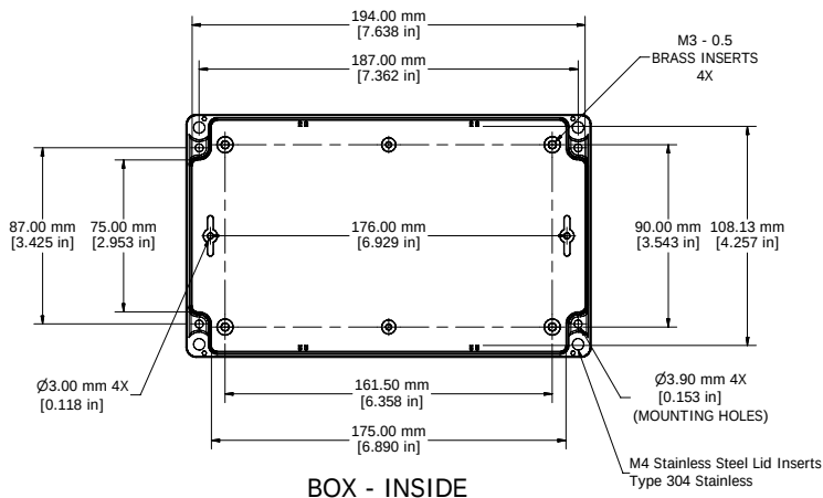
BOX - INSIDE
