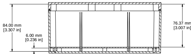
SECTION B-B
