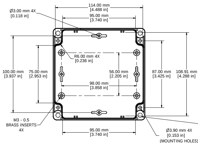
BOX - INSIDE
