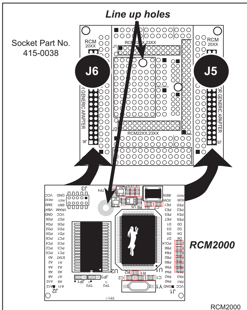
Figure 1. Top Side
