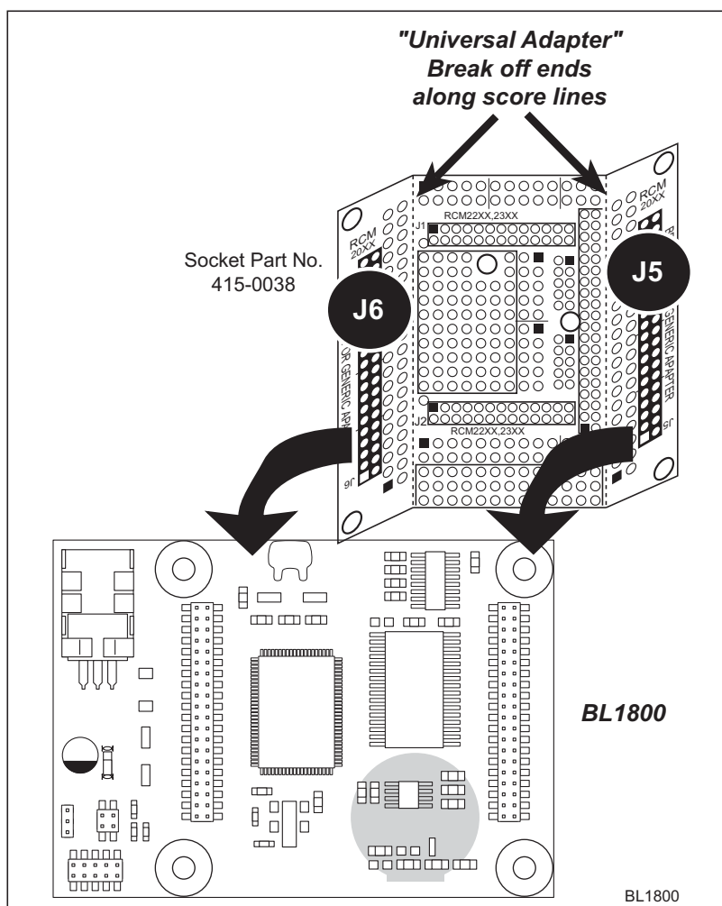
Figure 1. Top Side
