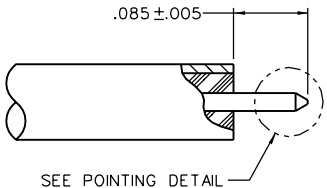
CABLE STRIP DIMENSIONS
