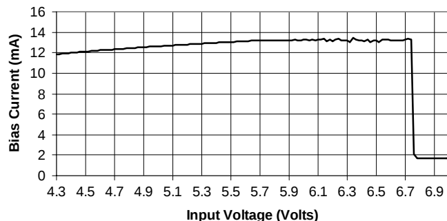
LDO Mode Bias Current vs Input Voltage
