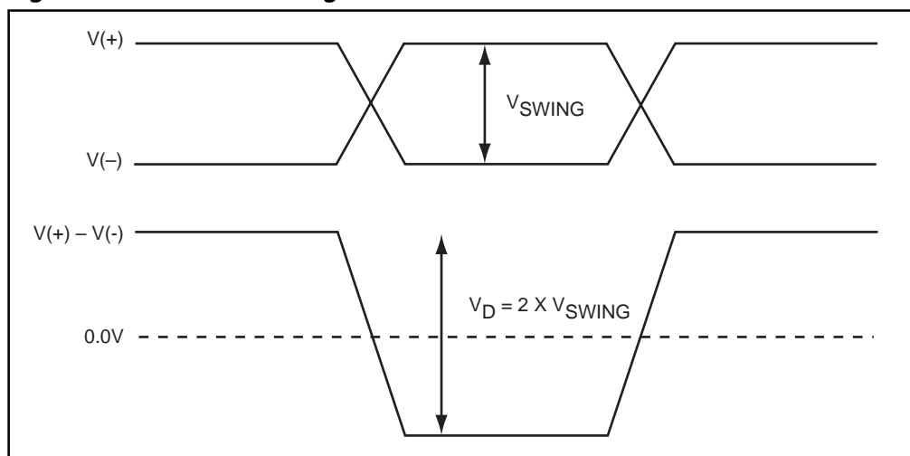
Figure 12. Differential Voltage Measurement
