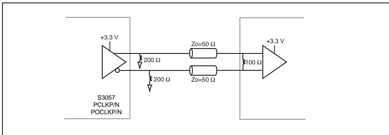
Figure 23. Differential LVPECL Driver to Differential LVPECL Input Termination 1
