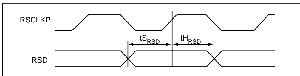
Figure 10. Receiver Input Timing Diagram
