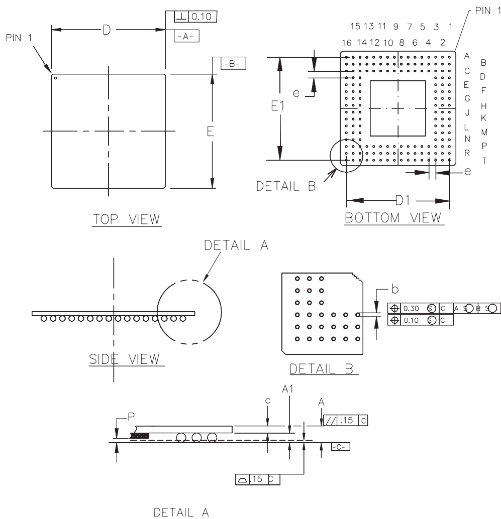
Figure 7. 156 TBGA Package
