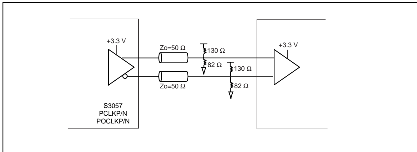
Figure 22. S3057 Differential LVPECL Driver to Differential LVPECL Input Termination
