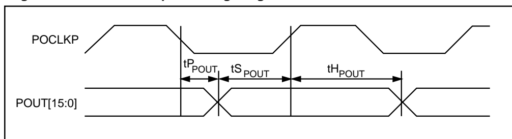
Figure 11. Receiver Output Timing Diagram
