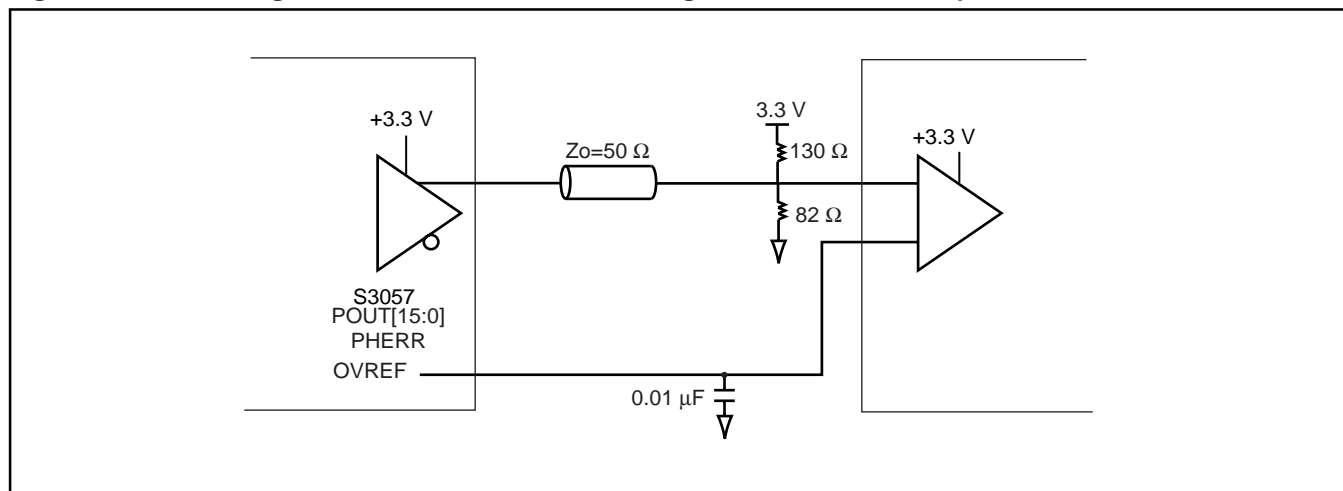
Figure 18. S3057 Single-Ended LVPECL Driver to Single-Ended LVPECL Input Termination
