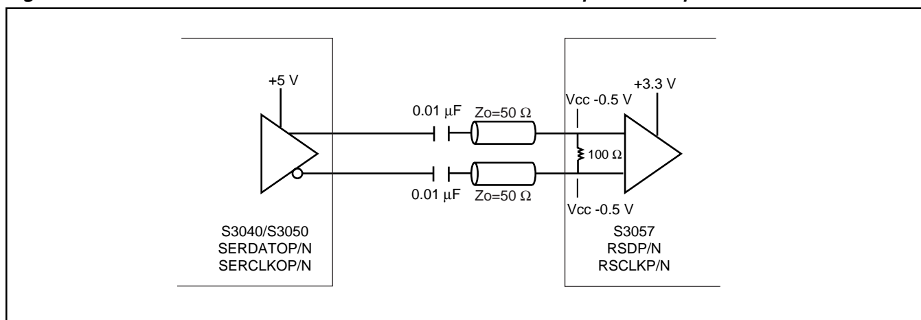
Figure 15. +5V Differential CML Driver to S3057 Differential CML Input AC Coupled Termination
