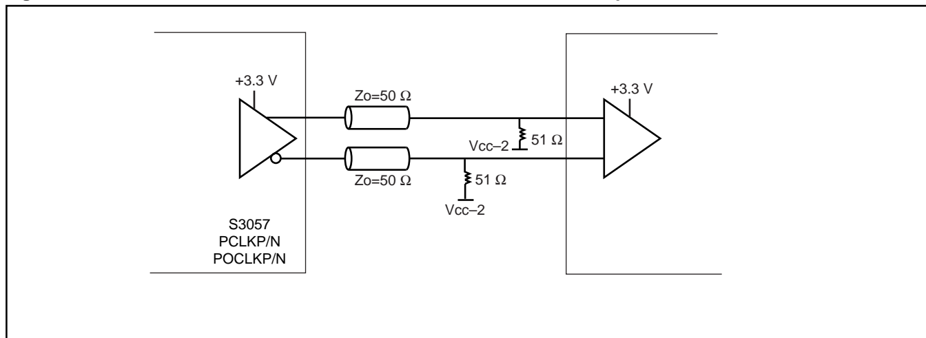
Figure 21. S3057 Differential LVPECL Driver to Differential LVPECL Input Termination
