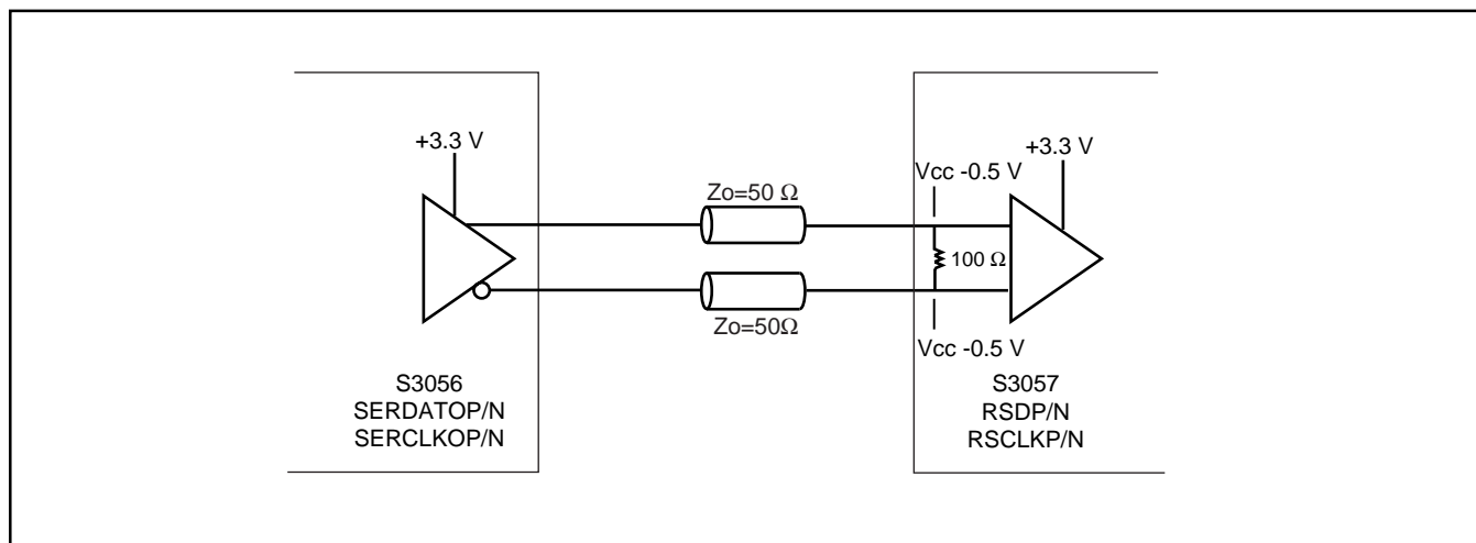
Figure 14. S3056 to S3057 Differential CML Input Termination
