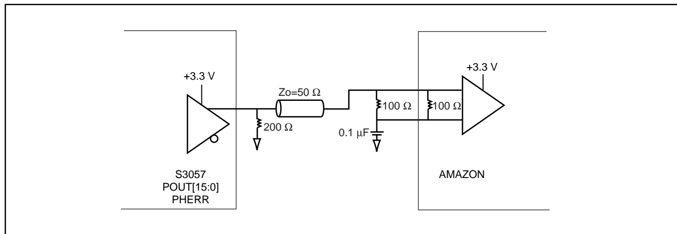
Figure 20. S3057 Single-Ended LVPECL Driver to Differential LVPECL Input Termination
