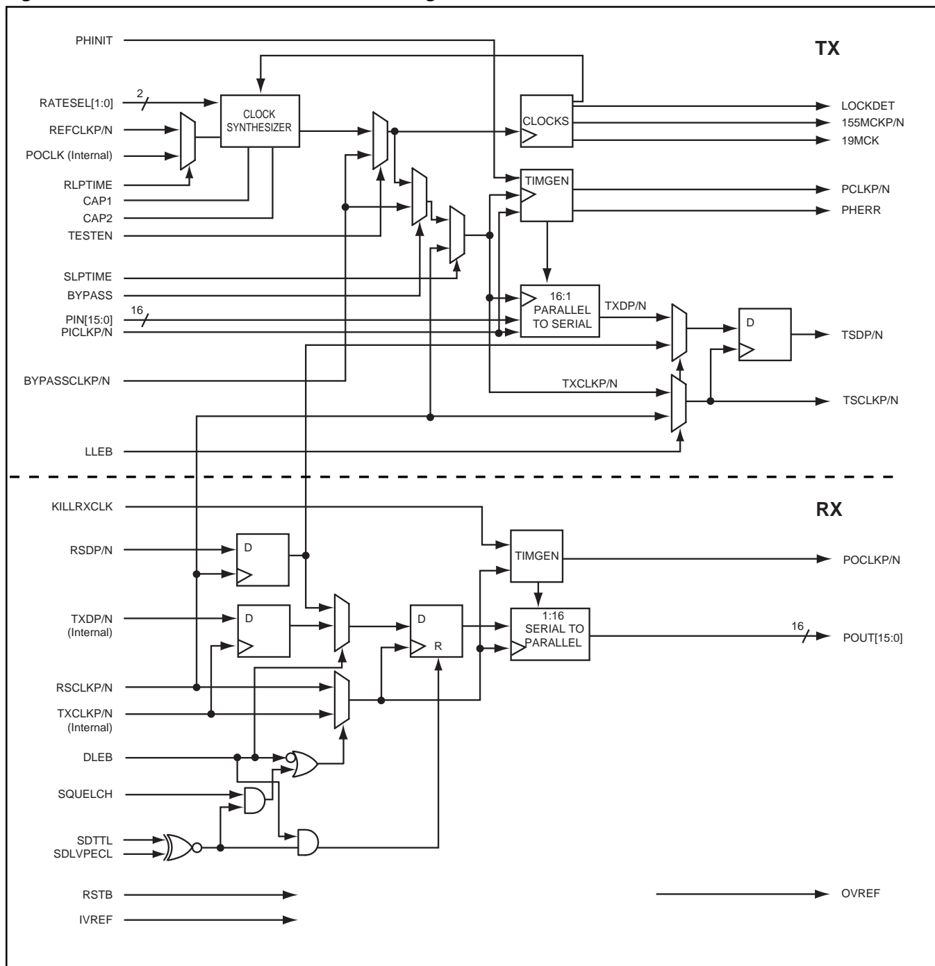
Figure 4. S3057 Transceiver Functional Block Diagram
