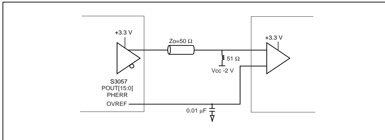
Figure 19. S3057 Single-Ended LVPECL Driver to Single-Ended LVPECL Input Termination
