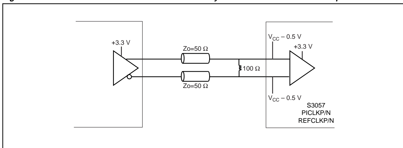
Figure 24. Differential LVPECL Driver to S3057 Internally Biased Differential LVPECL Inputs
