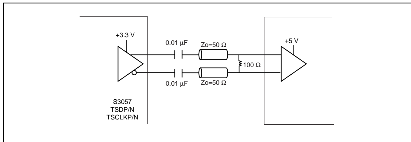
Figure 17. S3057 Differential CML Output to +5V PECL Input AC Coupled Termination
