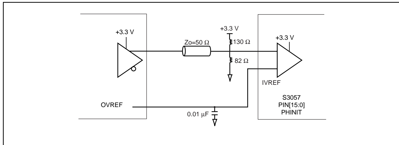
Figure 16. Single-Ended LVPECL Driver to S3057 Single Ended LVPECL Input Termination
