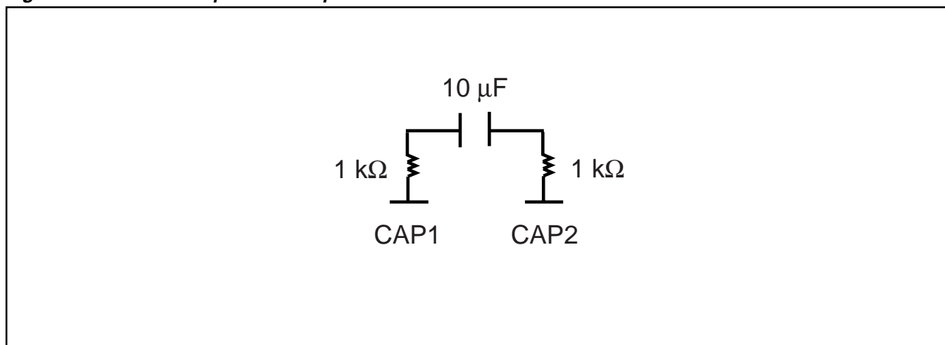
Figure 25. External Loop Filter Components
