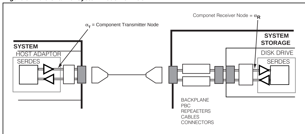
Figure 5. Fibre Channel System Node Definition
