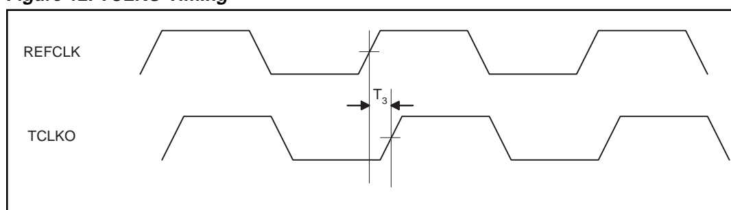
Figure 12. TCLKO Timing
