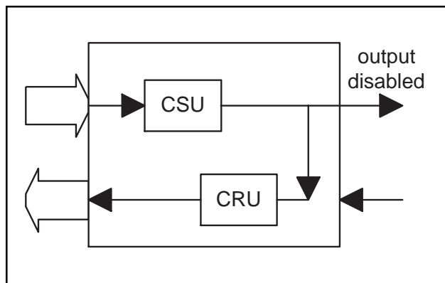
Figure 13. Loopback Operation
