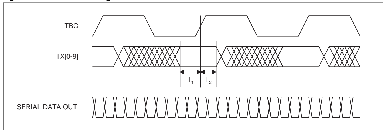
Figure 10. Transmitter Timing
