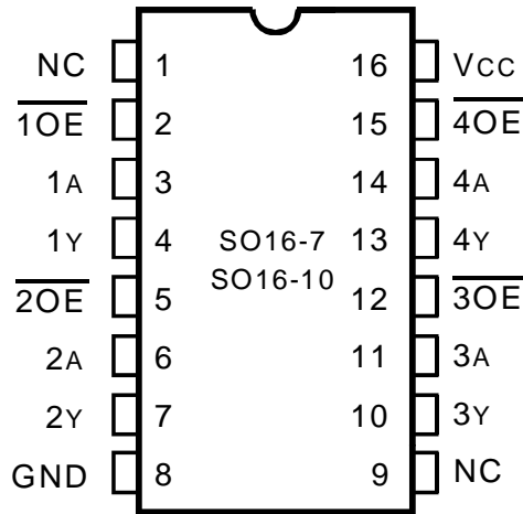
QSOP/TSSOP TOP VIEW
