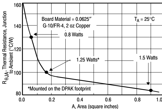
Figure 19. Thermal Resistance versus Collector Pad Area for the SOT-223 Package (Typical)
