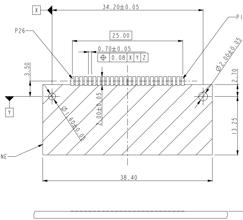
RECOMMENDED PCB LAYOUT (VIEW FROM MOUNTING SIDE)
