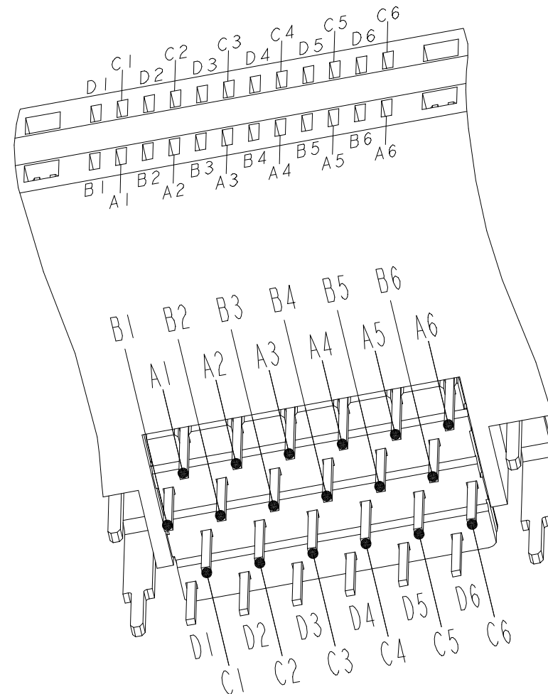
DETAIL F
