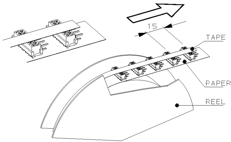
REEL PACKAGING DEREELING DIRECTION AND CONNECTOR POSITION. QUANTITY 2500 CONNECTORS PER REEL FOR ALL PARTNUMBERS, EXCEPT 4 POSITION 1500 CONNECTORS PER REEL.
