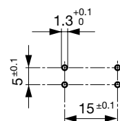
Drilling holes variants 0751.0052 and 0751.0062
