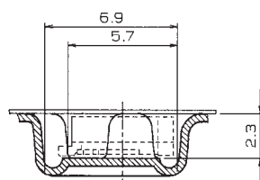
SECT. E-E
