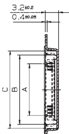
SECT. D-D
