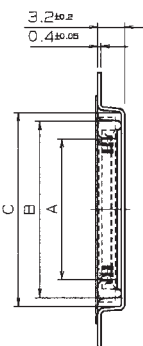
SECT. D-D
