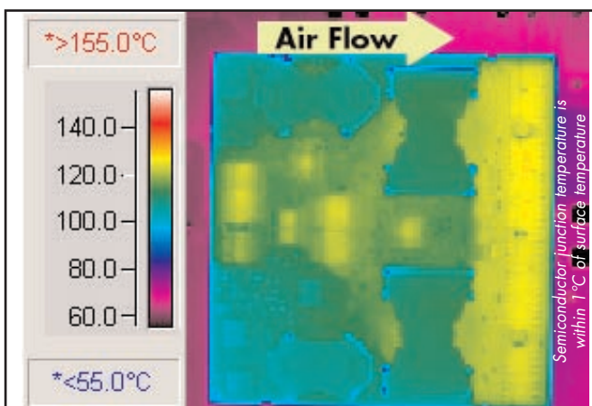
Figure 6: Thermal plot of converter at 44 amp load current with 55°C air flowing at the rate of 200 LFM. Air is flowing across the converter from input to output (nominal input voltage).
