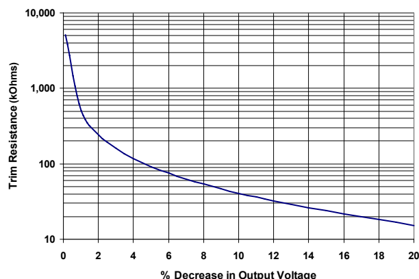
Figure B: Trim Down Graph for 1.8V out
