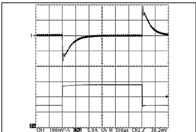
Figure 12: Output voltage response to step-change in load current (50%-75%-50% of I_{max} ; dI/dt = 5A/\mu s ). Load cap: 470μF, 30 mΩ ESR tantalum capacitor and 1μF ceramic capacitor. Top trace: V_{out} (100mV/div), Bottom trace: I_{out} (5A/div).
