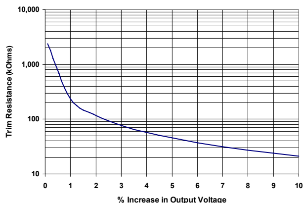
Figure C: Trim Up Graph for 1.8V out
