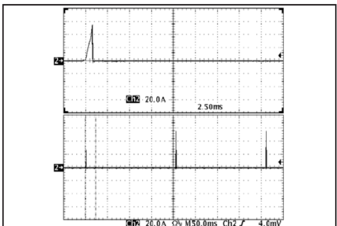
Figure 18: Load current (20A/div) as a function of time when the converter attempts to turn on into a 10\ \text{m}\Omega short circuit. Top trace is an expansion of the on-time portion of the bottom trace.
