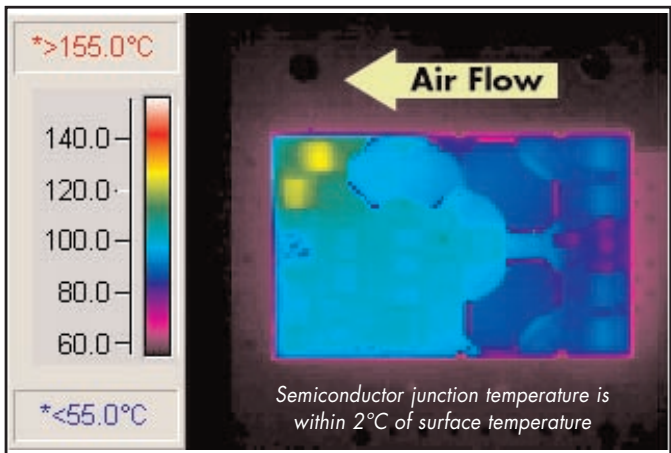
Figure 8: Thermal plot of converter at 25 amp load current with 55°C air flowing at the rate of 200 LFM. Air is flowing across the converter in the long direction from output to input (nominal input voltage).
