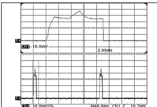
Figure 18: Load current (20A/div) as a function of time when the converter attempts to turn on into a 1\text{m}\Omega short circuit. Top trace (2ms/div) is an expansion of the on-time portion of the bottom trace.
