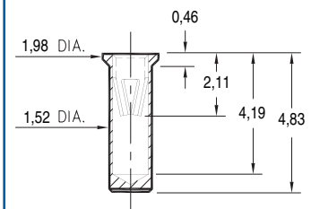
0415-0-15-XX-16-XX-10-0 Solder mount in 1,6 min. mounting hole Also available on 24mm wide carrier tape: 1,500 parts per 330mm reel. Order as: 0415-0-57-XX-16-XX-10-0
