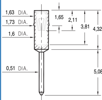
8114-0-15-XX-16-XX-04-0 Press-fit from underside of pc board into 1,65 mounting hole
