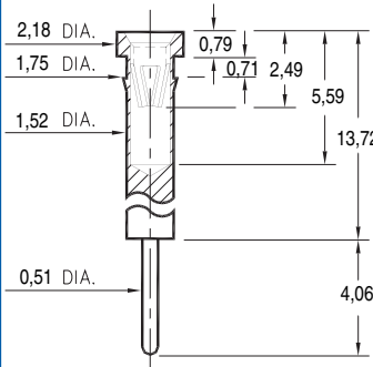
0407-0-15-XX-16-XX-04-0 Press-fit in 1,68 mounting hole
