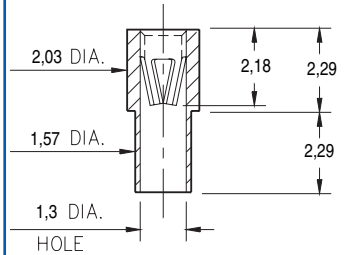
0285-0-15-XX-16-XX-10-0 Solder mount in 1,65 min. mounting hole
