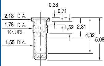
0293-0-15-XX-16-XX-10-0 Press-fit in 1,7 mounting hole
