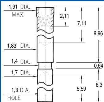
0306-0-19-XX-16-XX-10-0 Wire Termination #18 gage crimp barrel
