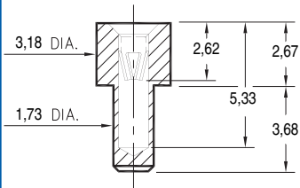
0284-0-15-XX-16-XX-10-0 Solder mount in 1,78 min. mounting hole
