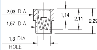
0287-0-15-XX-16-XX-10-0 Solder mount in 1,65 min. mounting hole Also available on 8mm wide carrier tape: 3,250 parts per 330mm reel. Order as: 0287-0-57-XX-16-XX-10-0
