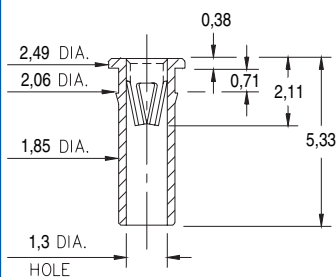
0273-0-15-XX-16-XX-10-0 Press-fit in 1,98 mounting hole
