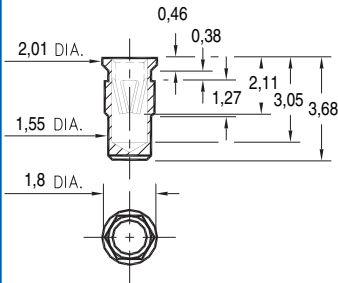
0291-0-15-XX-16-XX-10-0 Hex press-fit in 1,7 plated thru hole
