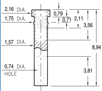
0303-0-19-XX-16-XX-10-0 Wire Termination Press-fit in 1,70 mounting hole
