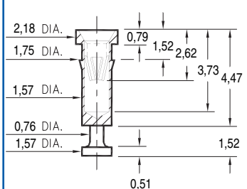
7520-0-15-XX-16-XX-10-0 Press-fit in 1,68 mounting hole
