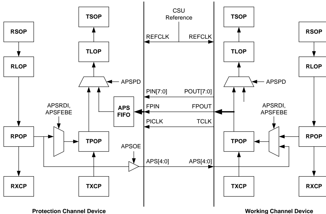
Figure 21: 1+1 APS Architecture
