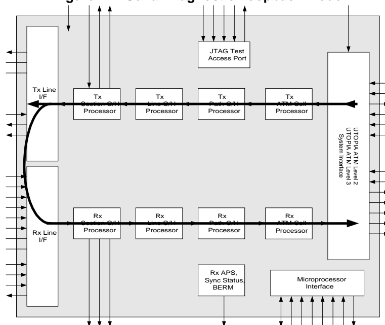
Figure 17: Serial Diagnostic Loopback mode
