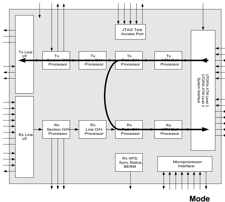
Figure 20: Data Diagnostic Loopback
