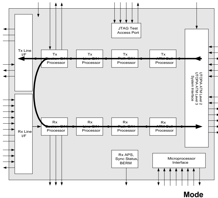
Figure 19: Path Diagnostic Loopback
