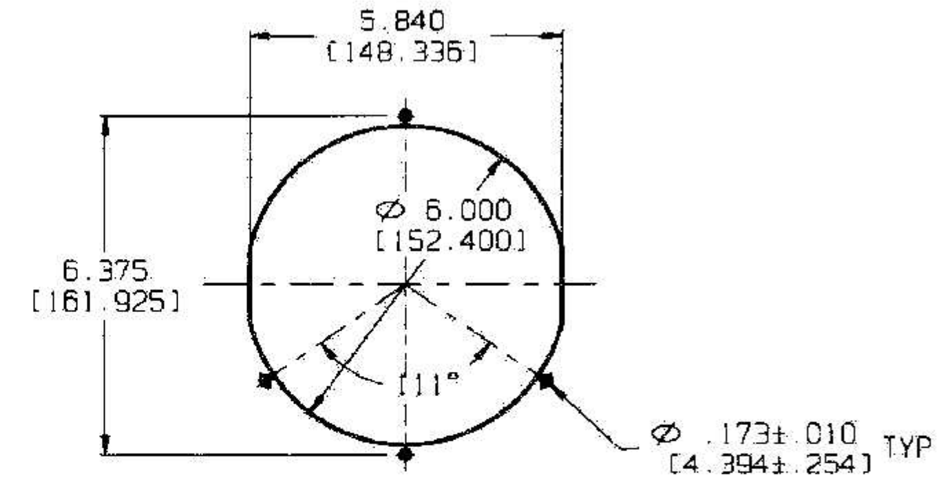
INLET (PROP) SIDE
