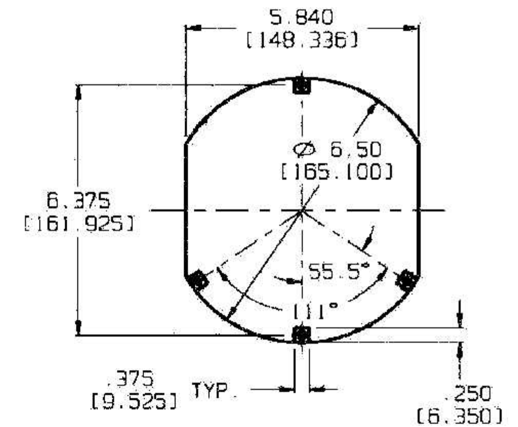
EXHAUST (STRUT) SIDE
