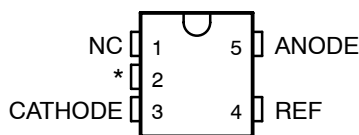
TLVH431 DBV (SOT-23-5) PACKAGE (TOP VIEW)
