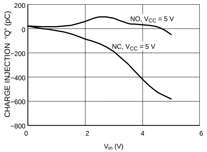
Figure 10. Charge Injection versus V_{in}
