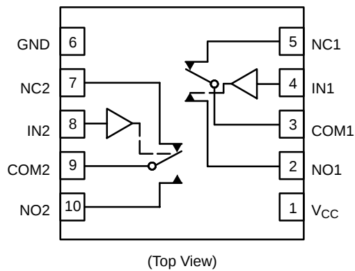
Figure 1. Pin Connections and Logic Diagram (QFN-10 and Micro10)
