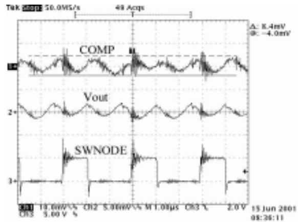
Figure 35. At Full-Load the Peak-to-Peak Voltage Ripple on the COMP Pin Should Be Less than 20 mV for a Well-Tuned/Stable Controller. Higher COMP Voltage Ripple Will Contribute to Output Voltage Jitter.
