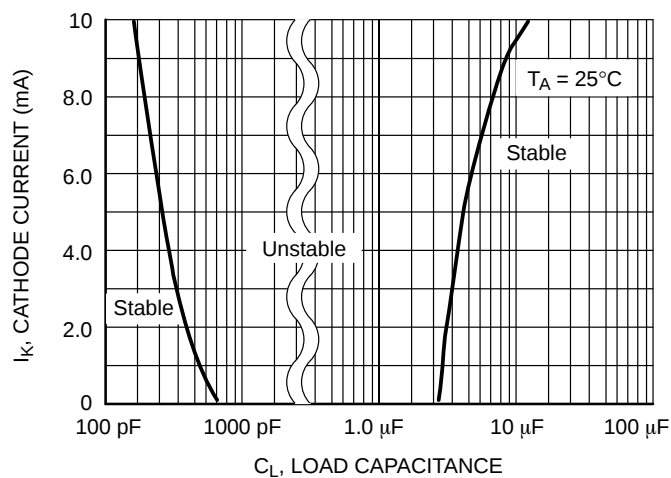
Figure 5. Reference Stability vs. Load Capacitance
