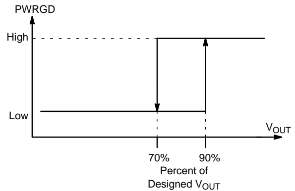
Figure 23. PWRGD Assertion
