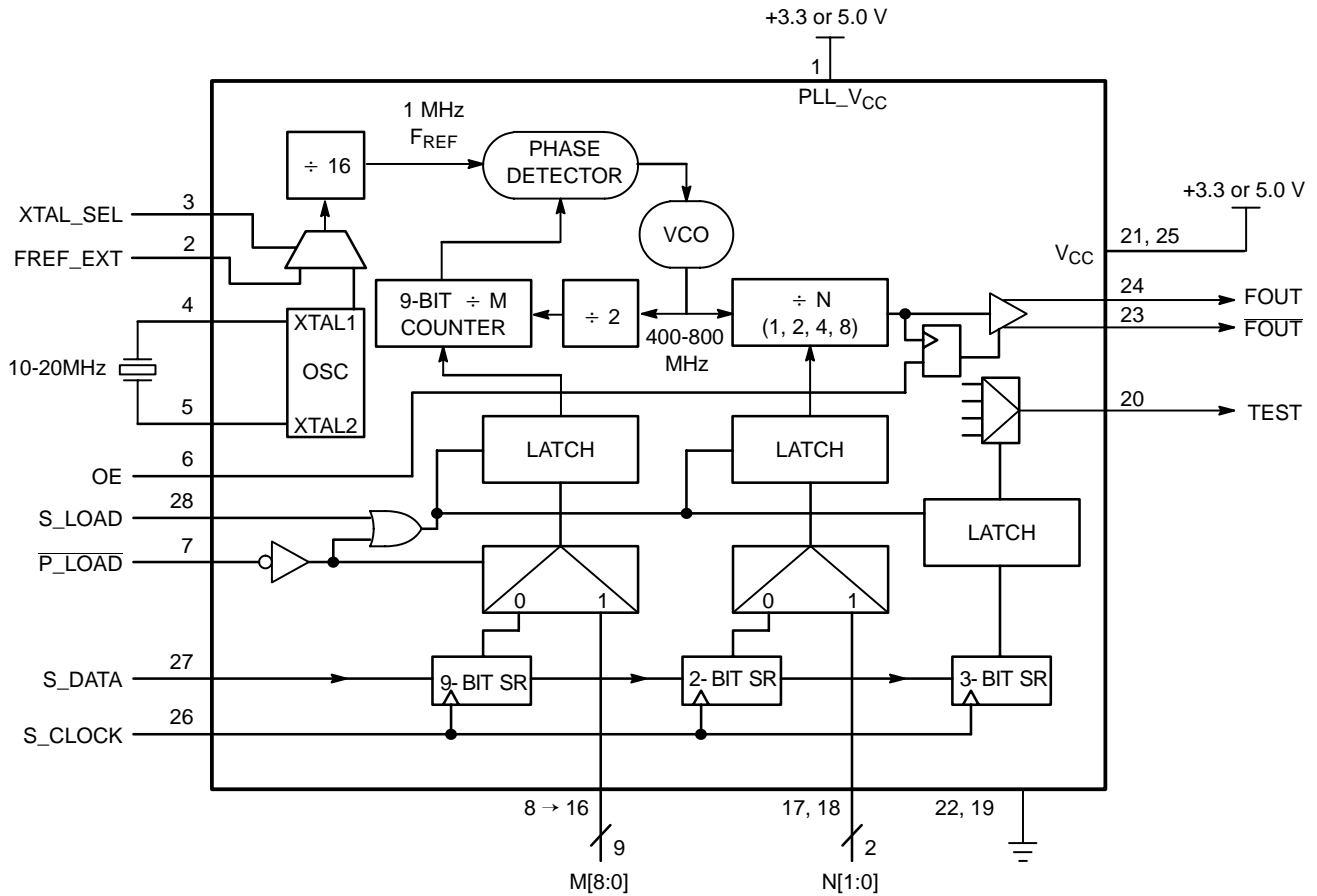
Figure 1. NBC12430 Block Diagram (28-Lead PLCC)
