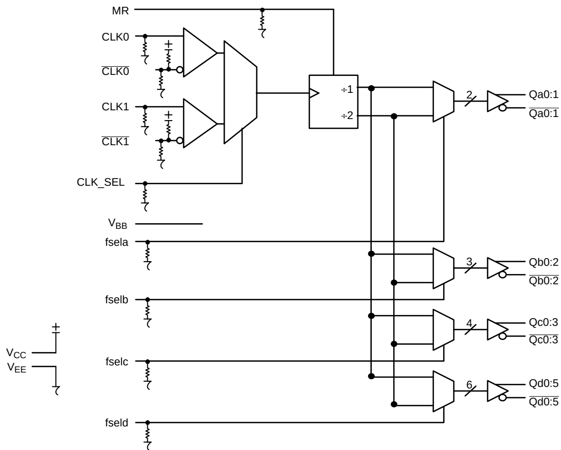
Figure 2. Logic Diagram
