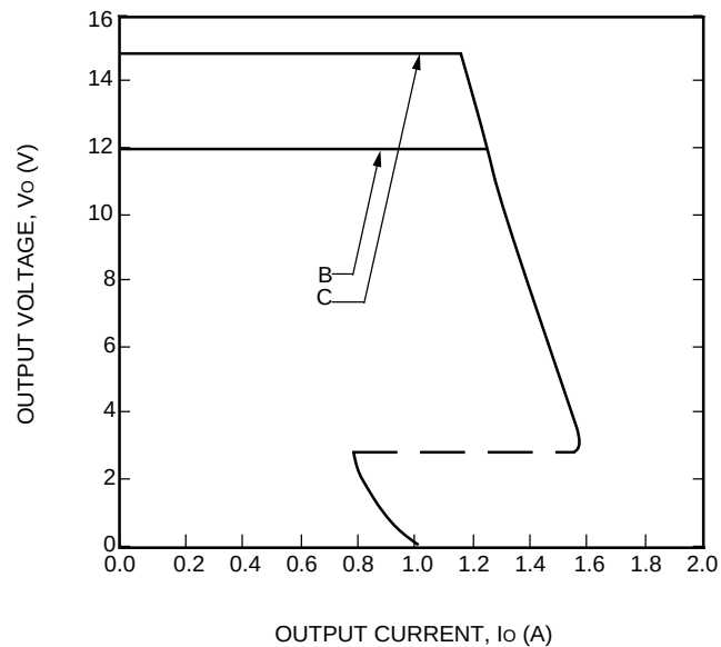
Figure 6. MW010B, C Typical Output Characteristic; V_i = 48 \text{ V} ; T_A = 25^\circ \text{C}
