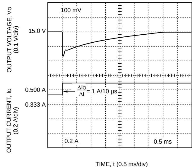
Figure 12. MW010C Typical Output Voltage Waveform for a Step Load Change from 50% to 75% of I_{o, \text{max}} ; V_i = 48 V; T_A = 25 °C
