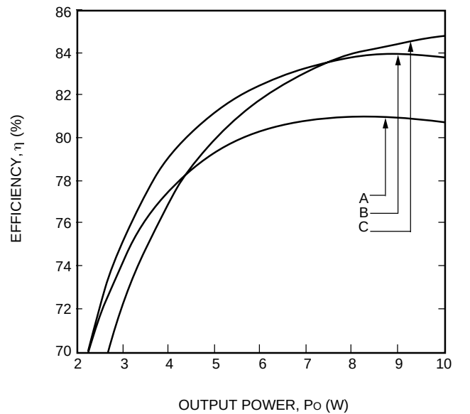
Figure 8. MW010A, B, C Typical Converter Efficiency as a Function of Output Power; V_i = 48 \text{ V} ; T_A = 25^\circ \text{C}
