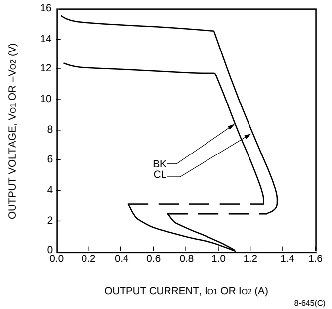
Figure 7. MW010BK, CL Typical Output Characteristic with One Output Fixed at Full Load; V_i = 48 \text{ V} ; T_A = 25^\circ \text{C}
