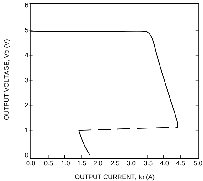
Figure 5. MW010A Typical Output Characteristic; V_i = 48 \text{ V} ; T_A = 25^\circ \text{C}
