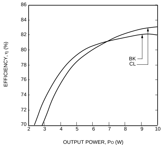
Figure 9. MW010BK, CL Typical Converter Efficiency as a Function of Output Power; V_i = 48 V; T_A = 25 °C
