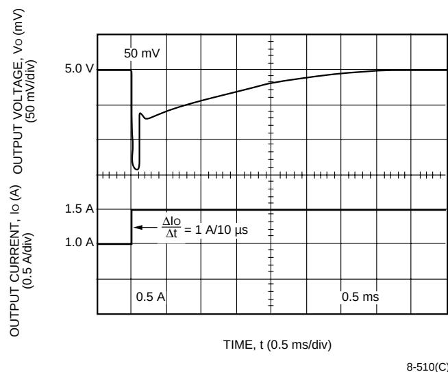
Figure 10. MW010A Typical Output Voltage Waveform for a Step Load Change from 50% to 75% of I_{o, \text{max}} ; V_i = 48 V; T_A = 25 °C
