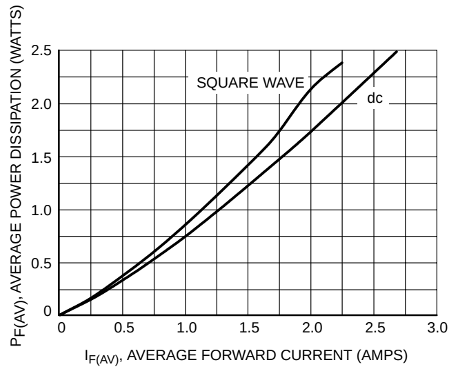
Figure 6. Power Dissipation
