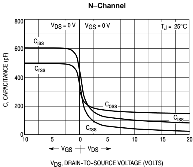
Figure 7. Capacitance Variation
