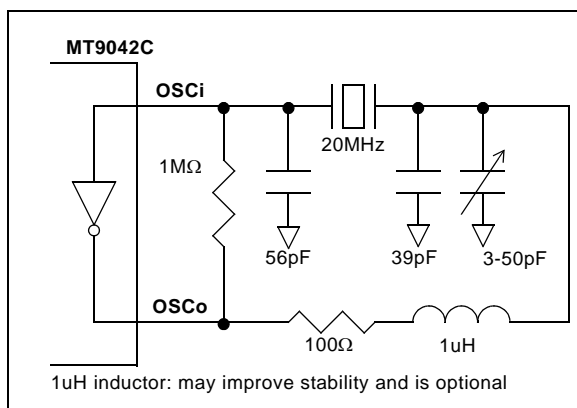
Figure 10 - Crystal Oscillator Circuit
