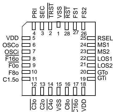
Figure 2 - Pin Connections
