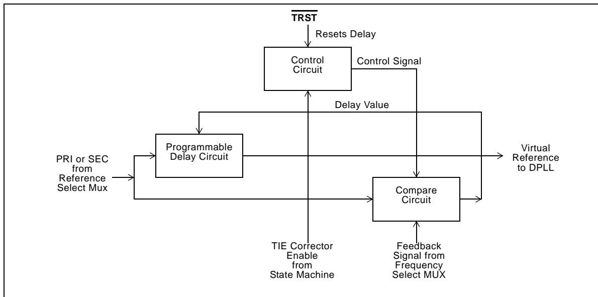
Figure 3 - TIE Corrector Circuit
