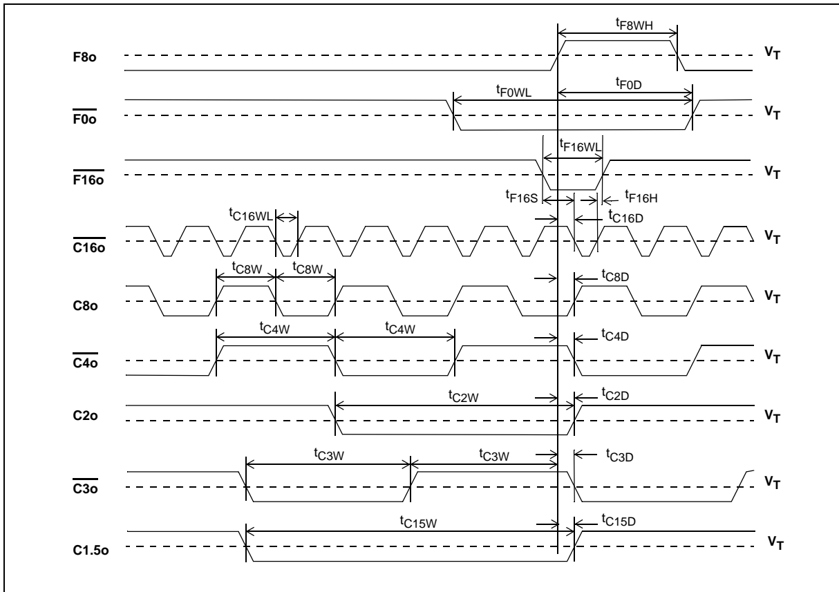
Figure 20 - Output Timing 1
