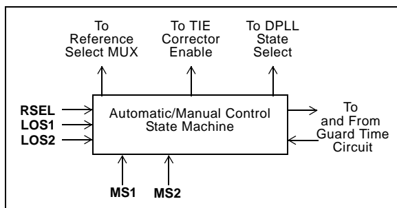
Figure 6 - Automatic/Manual Control State Machine Block Diagram
