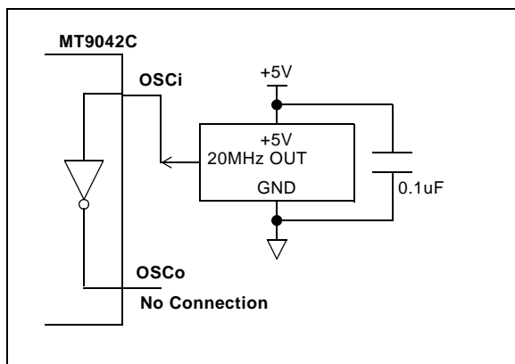
Figure 9 - Clock Oscillator Circuit
