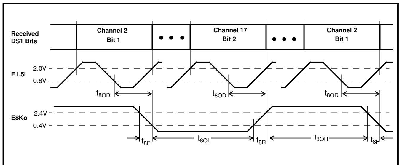
Figure 18 - E8Ko Timing
