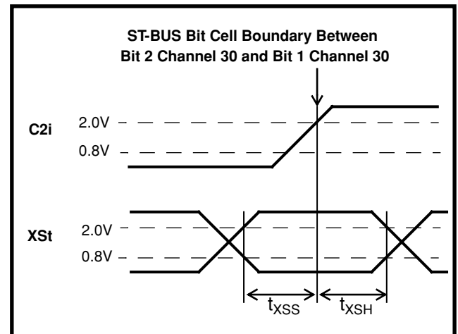
Figure 17 - XSt Timing
