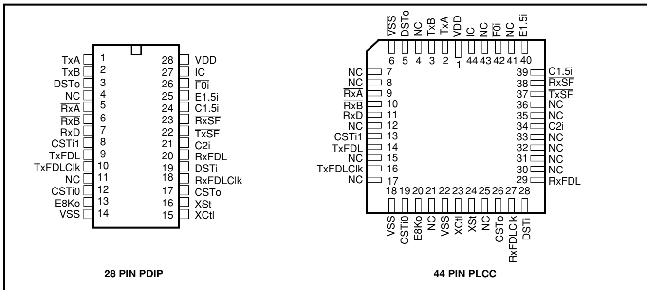
Figure 2 - Pin Connections
