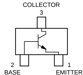
SC-59 CASE 318D STYLE 1
