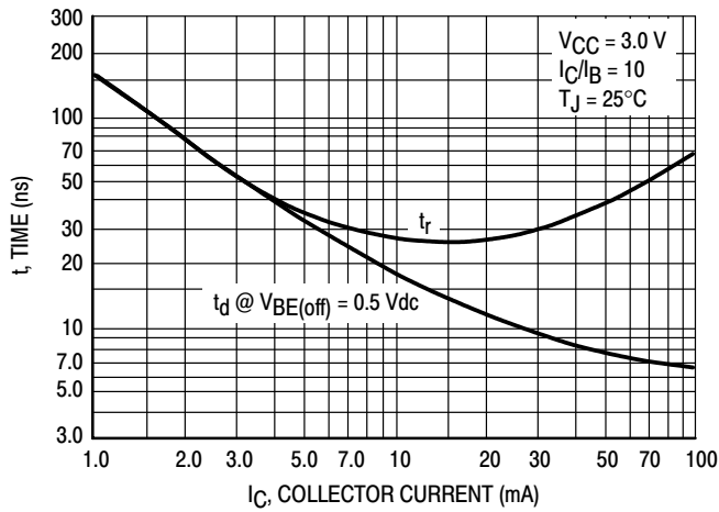
Figure 13. Turn-On Time
