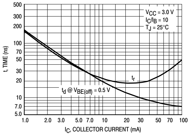
Figure 33. Turn-On Time
