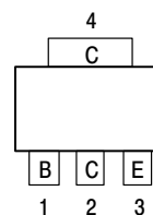
CASE 318E-04, Style 1
