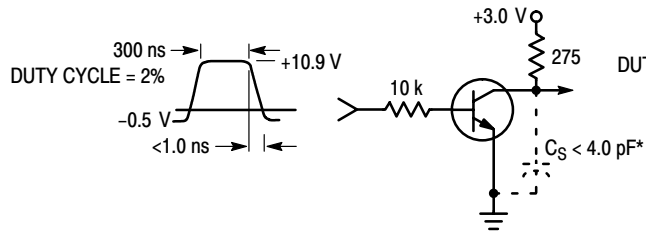
Figure 2. Turn-On Time
