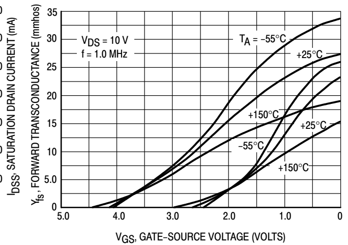
Figure 2. Forward Transconductance versus Gate-Source Voltage
