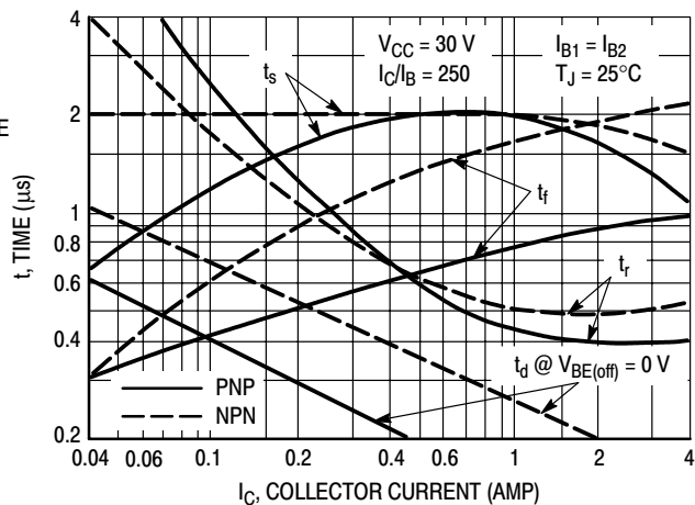
Figure 2. Switching Times
