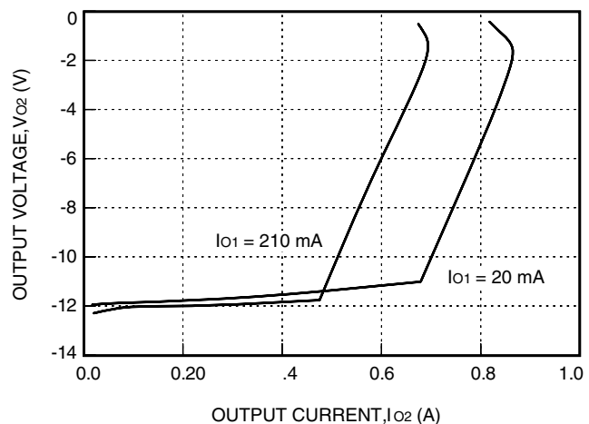
Figure 17. ME005BK Typical Output Characteristics ( V_{o2} vs. I_{o2} ) with V_i = 48 V and T_A = 25 °C
