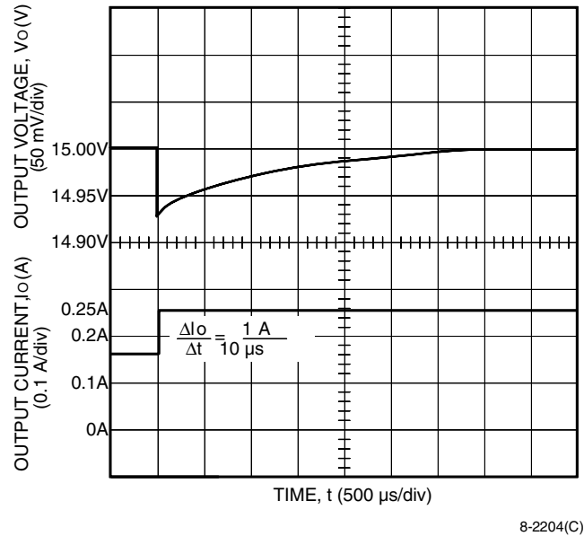
Figure 27. ME005C Typical Output Voltage Waveform for a Step Load Change from 50% to 75% of I_{o, \max} with V_i = 48 \text{ V} and T_A = 25^\circ \text{C}
