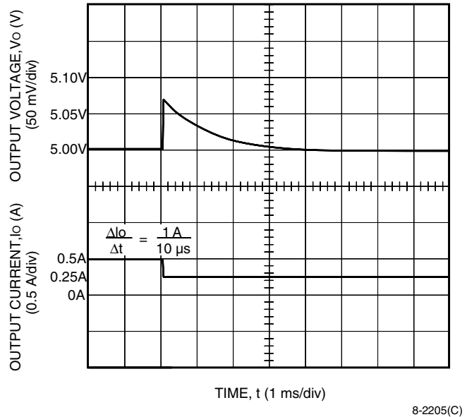
Figure 28. ME005A Typical Output Voltage Waveform for a Step Load Change from 50% to 25% of I_{o, \max} with V_i = 48 \text{ V} and T_A = 25^\circ \text{C} (ME005N Waveform Is Similar, but with 5.2 V Steady-State.)
