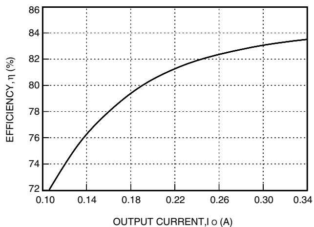
Figure 22. ME005C Typical Converter Efficiency as a Function of Output Current with V_i = 48 V and T_A = 25 °C
