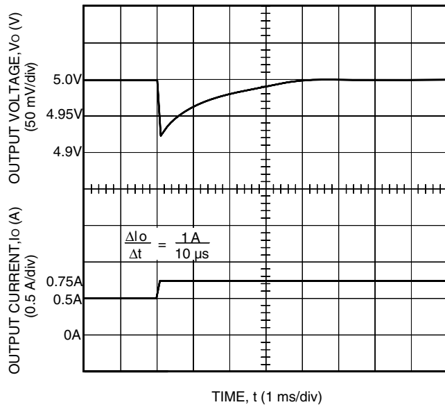
Figure 25. ME005A Typical Output Voltage Waveform for a Step Load Change from 50% to 75% of I_{o, \max} with V_i = 48 \text{ V} and T_A = 25^\circ \text{C} (ME005N Waveform Is Similar, but with 5.2 V Steady-State.)
