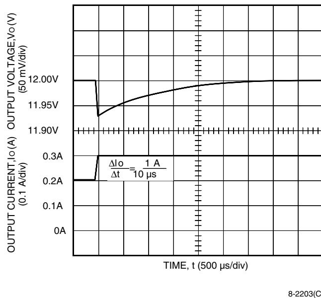
Figure 26. ME005B Typical Output Voltage Waveform for a Step Load Change from 50% to 75% of I_{o, \max} with V_i = 48 \text{ V} and T_A = 25^\circ \text{C}
