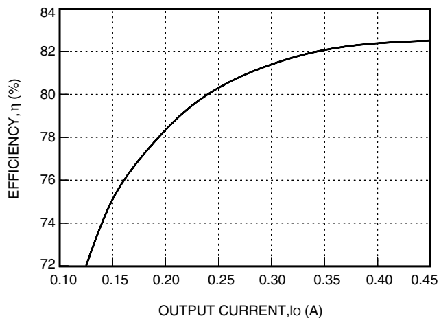
Figure 21. ME005B Typical Converter Efficiency as a Function of Output Current with V_i = 48 V and T_A = 25 °C
