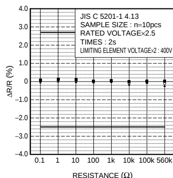
Fig.7 Overload
