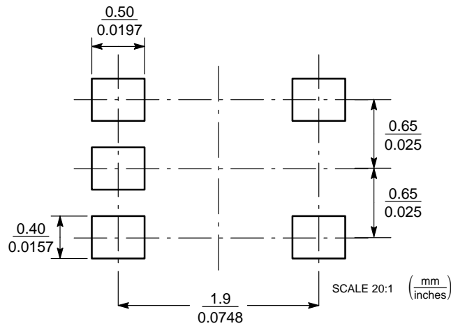
Figure 11. SC-88A/SC70-5/SOT-353
