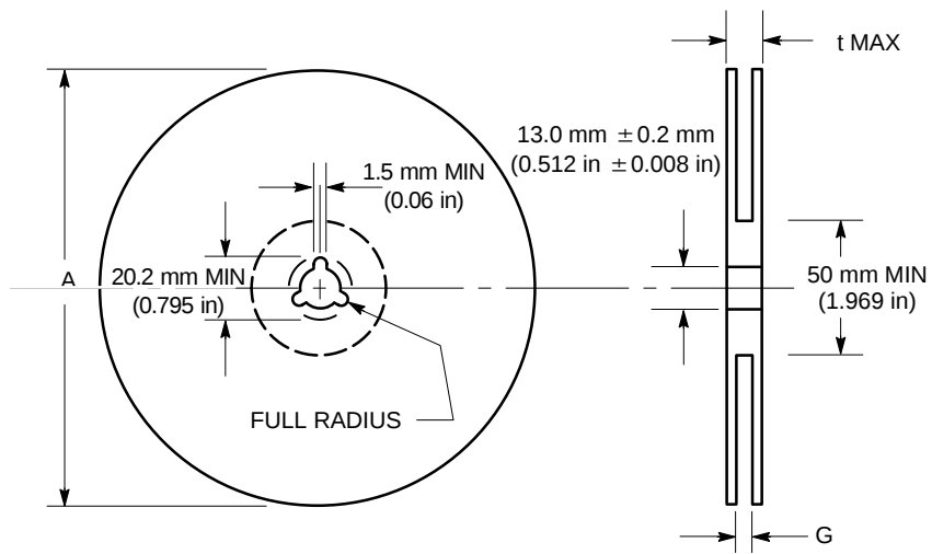
Figure 19. Reel Dimensions
