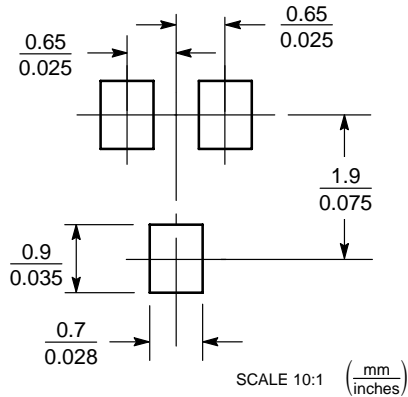
Figure 11. SC-70/SOT-323
