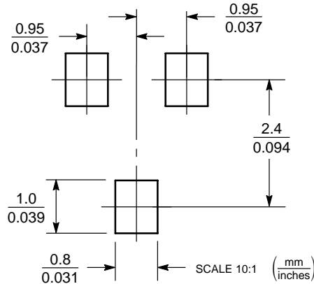
Figure 12. SC-59
