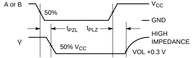
Figure 5. Switching Waveforms
