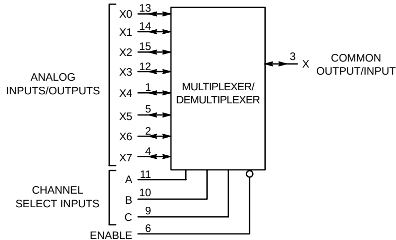
Single-Pole, 8-Position Plus Common Off
