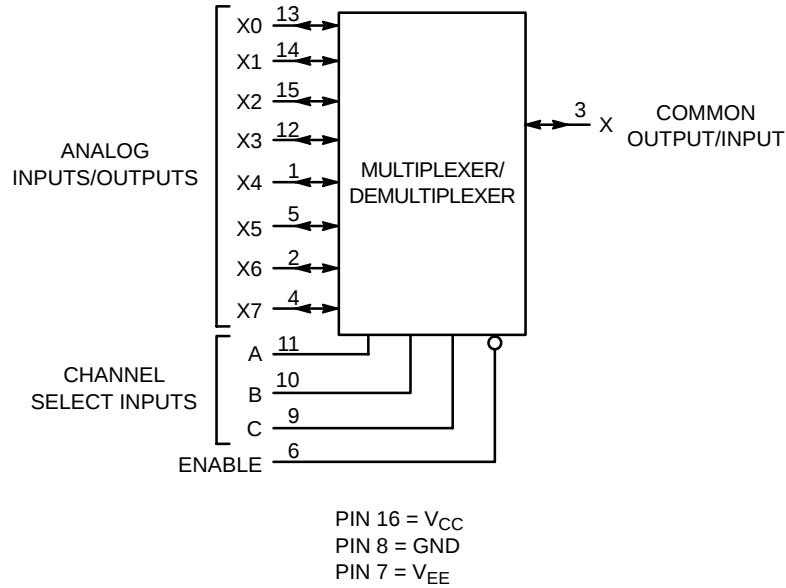
Figure 2. Logic Diagram
