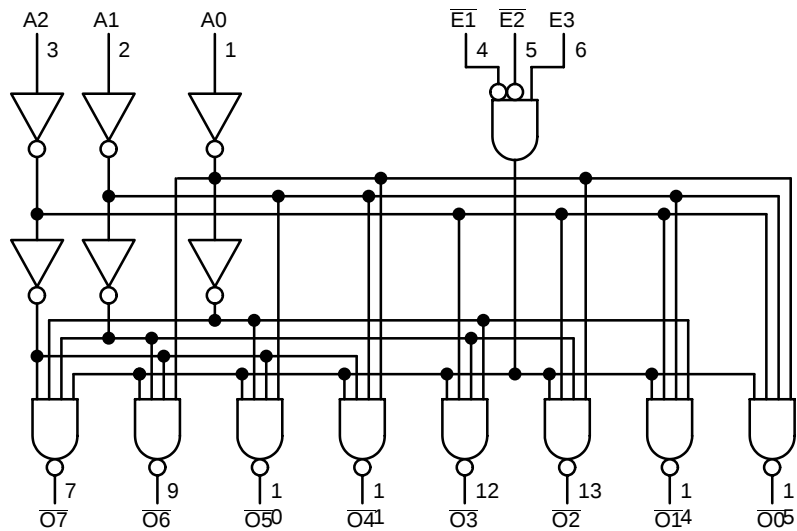
Figure 2. Logic Diagram
